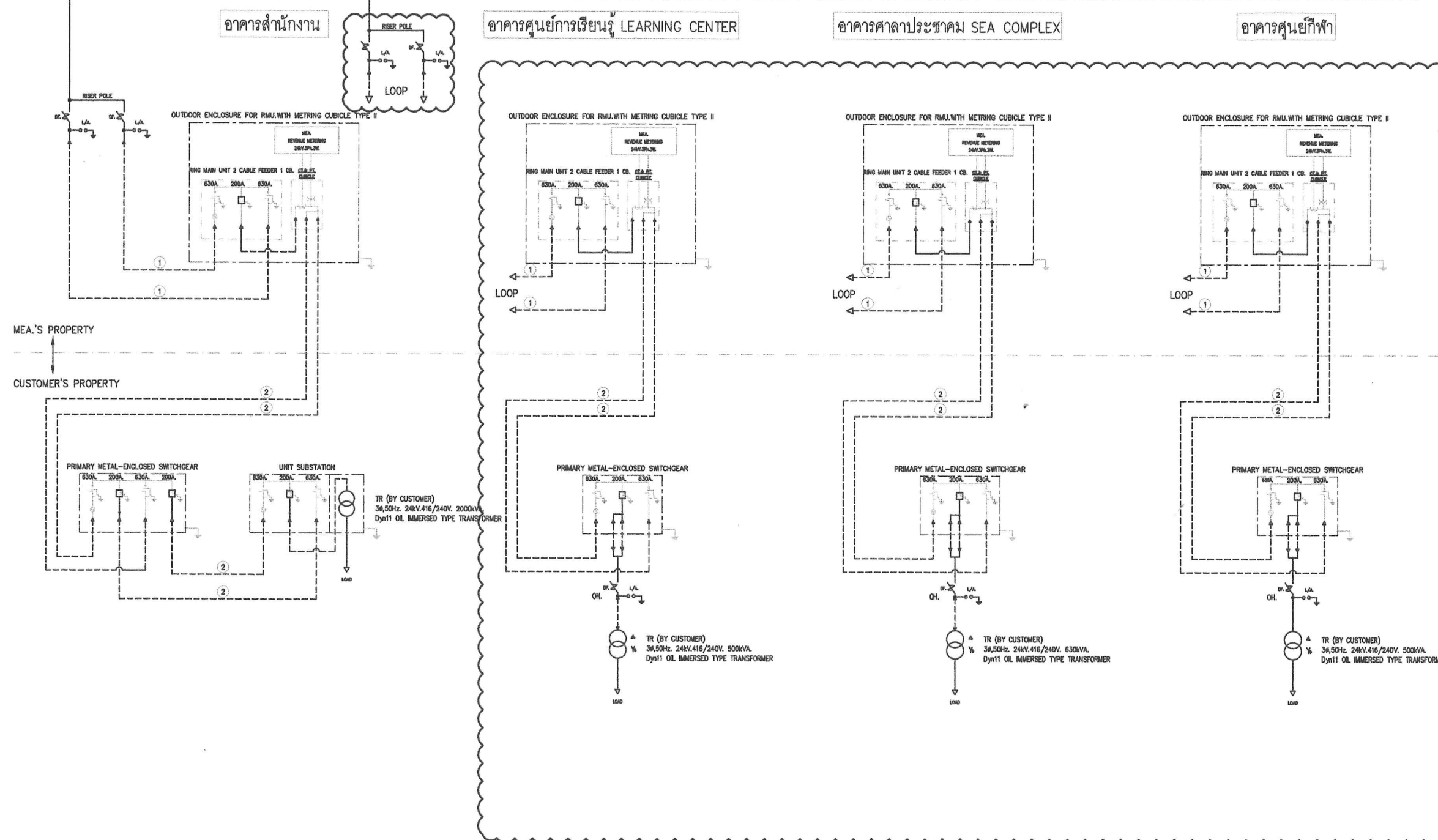
SINGLE LINE DIAGRAM FOR HIGH VOLTAGE
